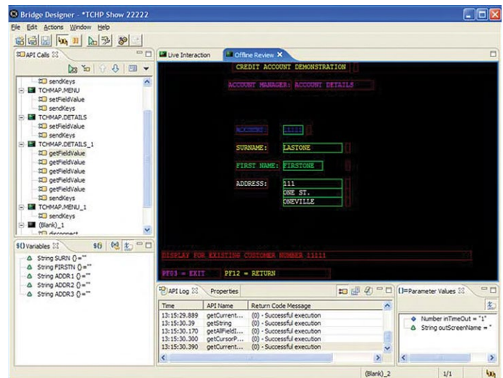
Fig 1. The Verastream bridge designer lets developers abstract bridge interactions using an interface that mirrors a 3270 session for ease of use
