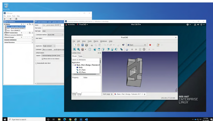
Fig 1. From Windows you can view Linux desktops configured for the Gnome 3 desktop.
