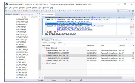
ASG-JOB/SCAN within the IBM IDz IDE, available with the DevOps Enablement package
