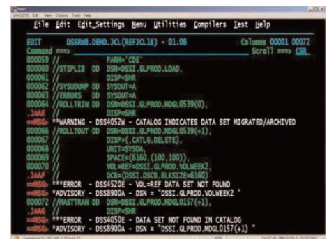
Standard ASG-JOB/SCAN within ISPF
