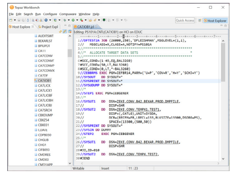
ASG-PRO/JCL within the Compuware Topaz Workbench IDE
