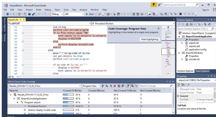
Figure 4. Feature-rich IDEs support rapid application development of COBOL systems for both mainframe and distributed platform deployment.
