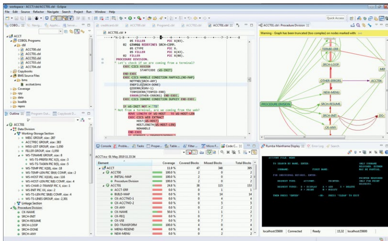
Figure 3. Rocket development tooling supports creation of mainframe and distributed COBOL applications.
