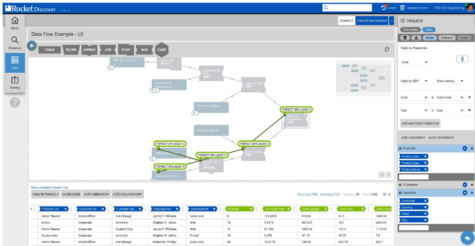
Figure 1. Graphical User Interface
