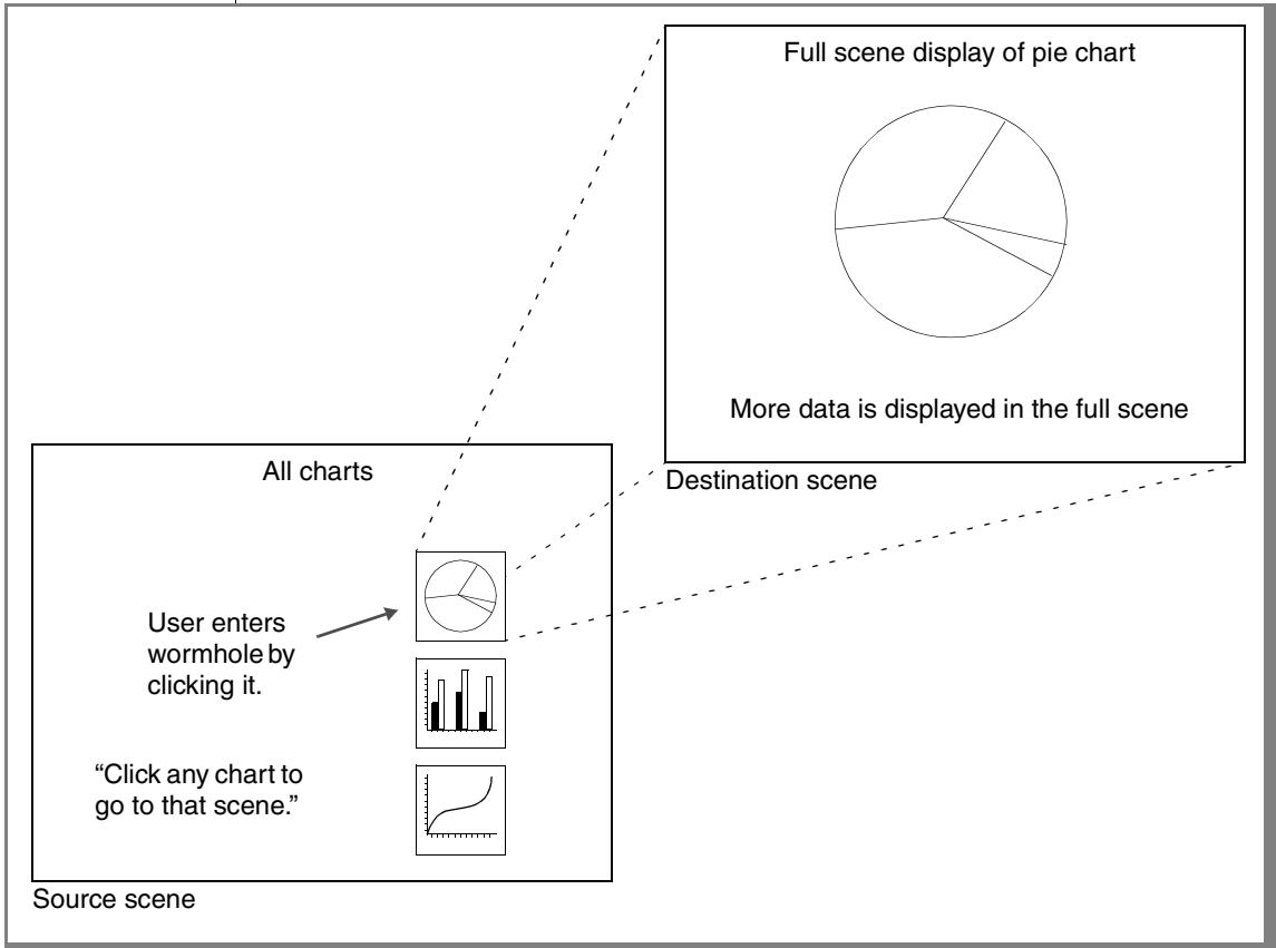
Figure 5-1 Wormhole
