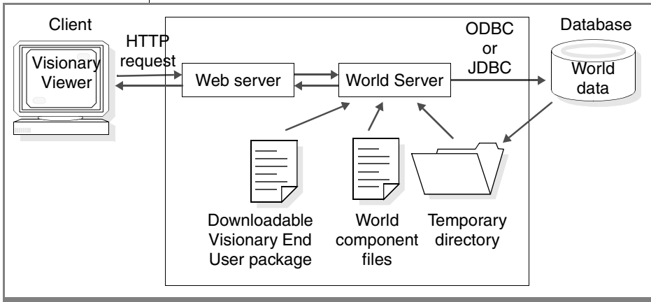
Figure 8-5 Internet Deployment Architecture
